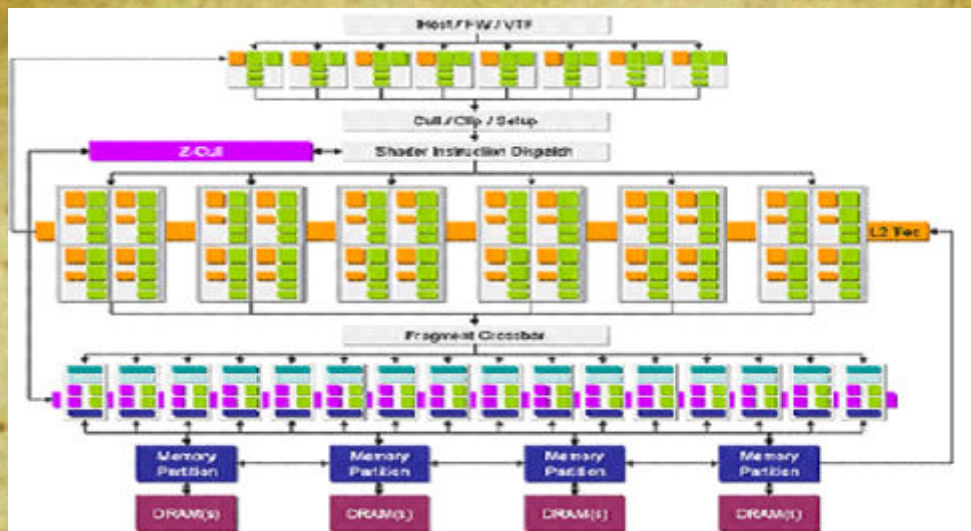
Fig2. Architecture of GeForce 7800
