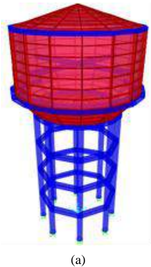
Fig 4. (a) FE model of elevated water tank using SAP 2000 (b) Arrangement of different type of column on outer periphery of staging
