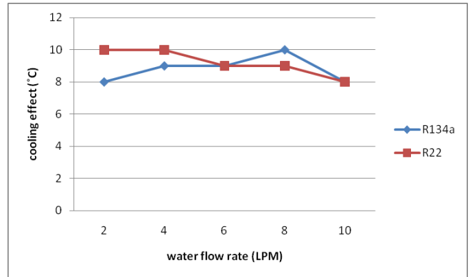
Fig.9 cooling effect (°C) vs water flow rate through condenser ( evaporator water flow rate constant)
