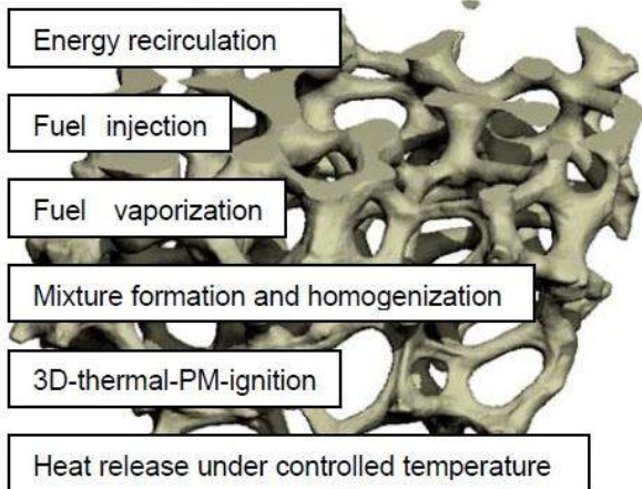
Figure 5: The important engine processes that may be supported by the PM technology
