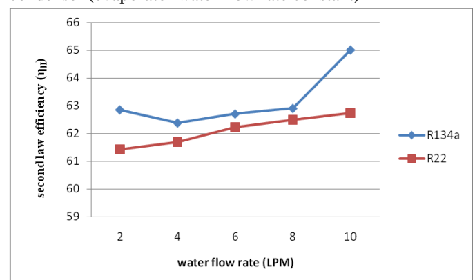
Fig.6 second law efficiency vs water flow rate through evaporator ( condensr water flow rate constant)
