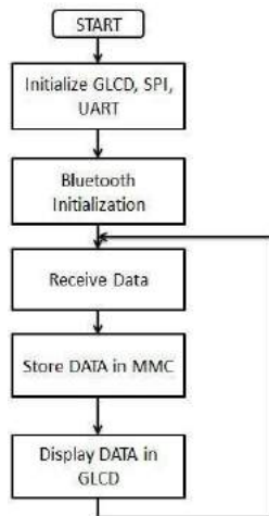
Fig. 8: Receiver Flowchart
