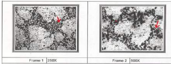
Figure 1: Unalloyed A-356
