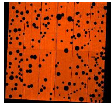
Fig. 7 (b) Images of background of X-ray Astronomical objects
