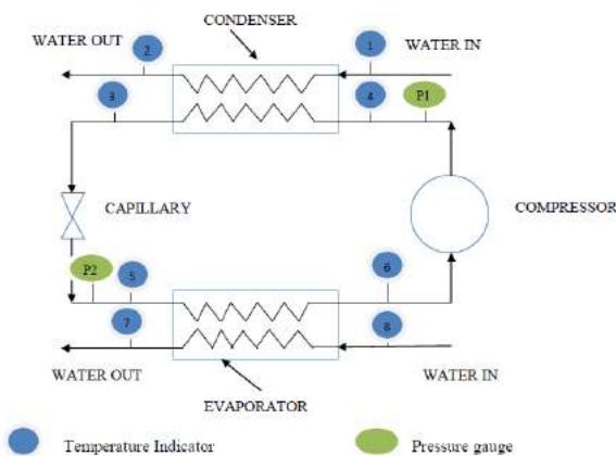
Fig.1 Schematic diagram of test rig.
