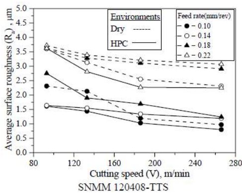
Figure 11: Variation in surface roughness with cutting speeds at different feeds under dry and HPC conditions
