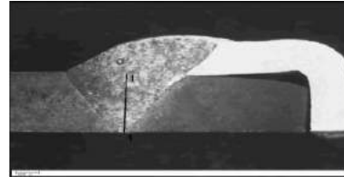
Fig. 9 Weld Penetrations for Sample S3
