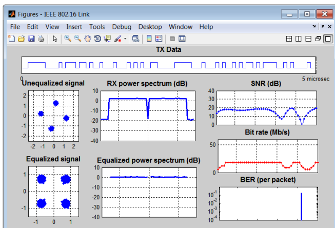
Fig.9 Effect of flat-fading channel on received and equalized signal
