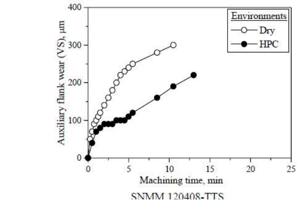
Figure 6: Growth of average auxiliary flank wear (VS) with machining time under dry and HPC conditions
