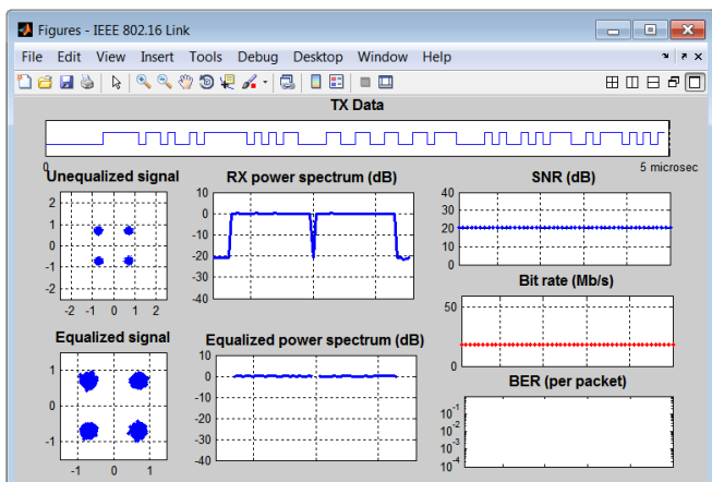
Fig.8 Effect on received and equalized signal when there is no fading.
